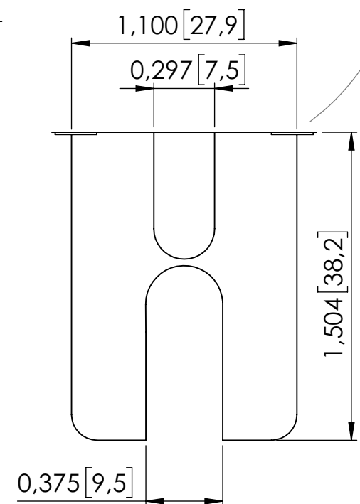
DETAIL VIEW
