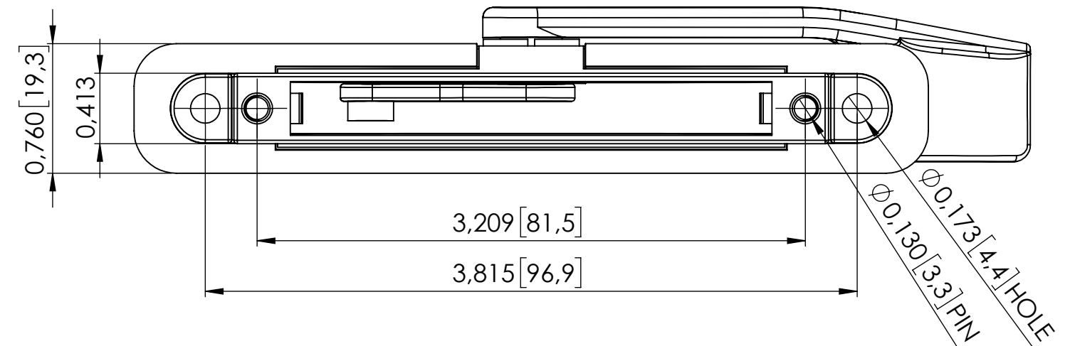
BOTTOM VIEW
