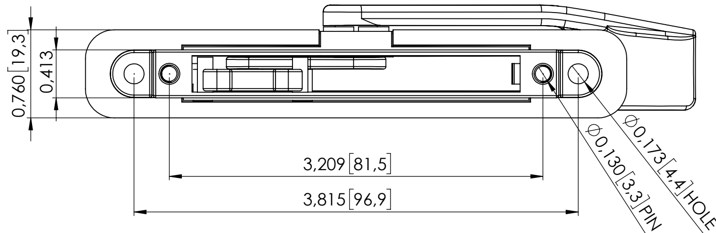
BOTTOM VIEW
