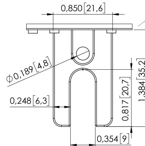
DETAIL VIEW
